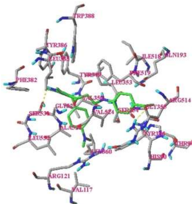
Fig. 7. Binding mode of compound 2c into binding site of COX-II, Showing two H-bonds with the guanido side chain of Arg514. Significant hydrophobic contact is found between the pyrimidine thione moiety of the compound with the side chains of Trp388, Tyr386, Phe519 and Met523. Furthermore, the side chains of Leu532, Val117, Leu360 and Val350 with the N,N- dimethylaniline moiety also show hydrophobic contact
