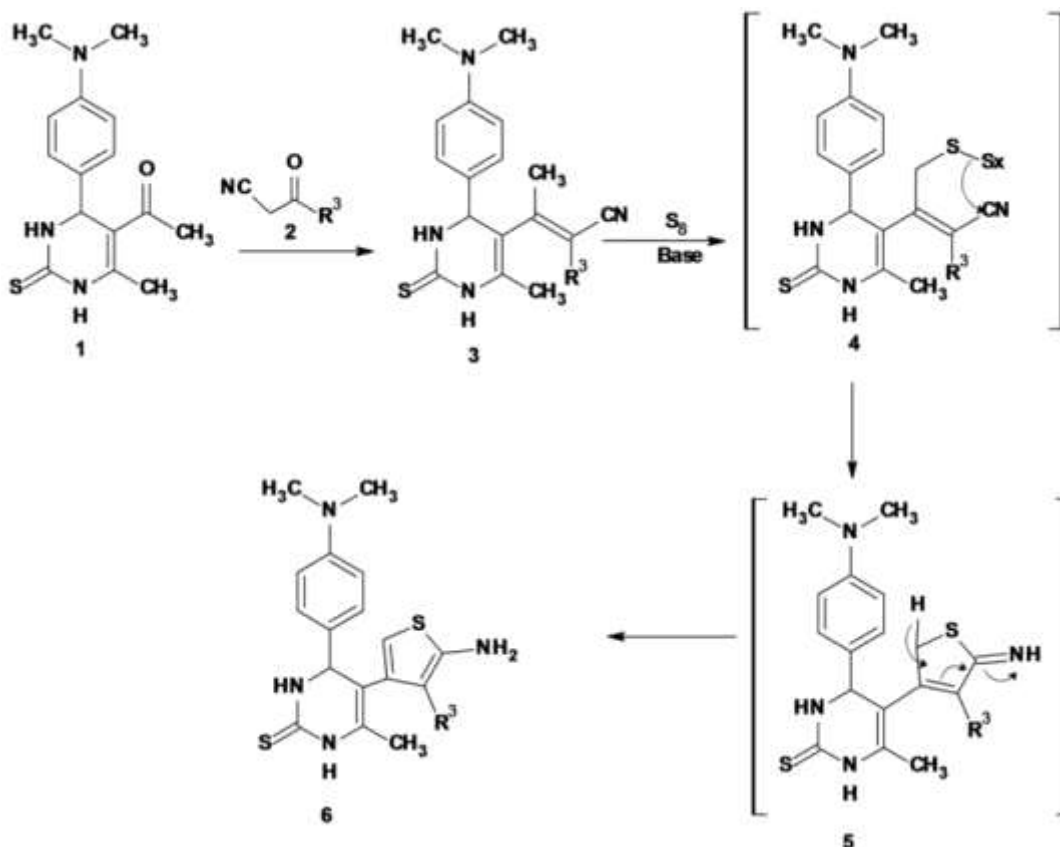
Fig. 4.Synthetic and mechanistic pathway for preparation of thiopyrimidines 7a,b
